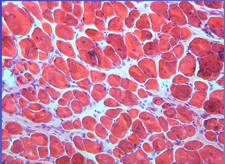
MMP9/PIGF Treat
