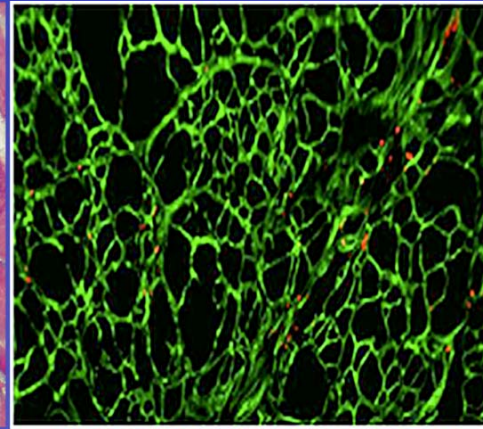
Laminin/CD11b
