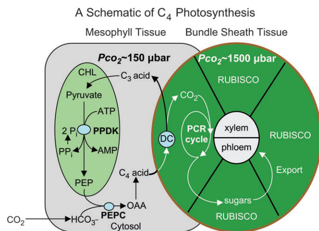
Fig. 1. A schematic diagram of the C_4 photosynthetic pathway showing the coupling of the C_4 cycle that originates in the mesophyll, and the C_3 cycle that originates with the fixation of CO_2 by Rubisco in the bundle-sheath compartment. Arrows indicate the path of molecule diffusion. Abbreviations: DC, decarboxylating enzyme; PEPC, PEP carboxylase; PCR, photosynthetic carbon reduction; PDK, pyruvate, phosphate dikinase.
