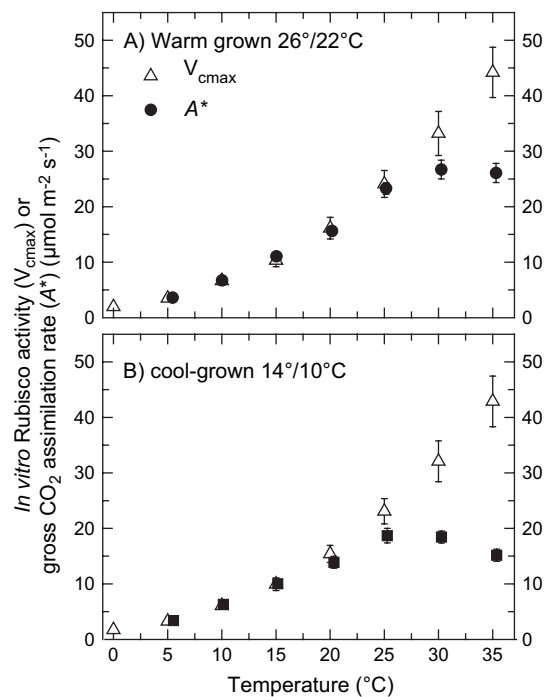
Fig. 6. The response of the maximum Rubisco activity ( V_{cmax} ) determined in vitro as a function of assay temperature, and the gross photosynthesis rate ( A^* ) measured with gas exchange in the C_4 grass Muhlenbergia glomerata . (A) M. glomerata grown at 26 °C during the day and 22 °C at night in a plant growth chamber. (B) M. glomerata grown at 14/10 °C day/night temperature. Plants were grown at 800 \mu mol photons m^{-2} s^{-1} . Note: photosynthesis and Rubisco activities are the same below 20 °C, but not at the thermal optimum. Rubisco contents for each treatment are not statistically different. From Kubien and Sage (2004a); with kind permission of Blackwell Publishing.
