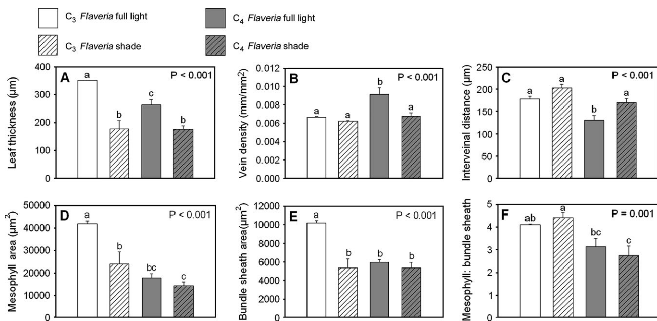
Fig. 5. Quantitative anatomical data from Flaveria robusta ( C_3 ) and Flaveria australasica ( C_4 ) grown under illuminated ( 500 \mu\text{mol m}^{-2} \text{s}^{-1} , red:far red ratio of 1.55) and shaded ( 100 \mu\text{mol m}^{-2} \text{s}^{-1} , red:far red ratio of 0.5) conditions in a plant growth chamber. All leaves sampled were at maturity, and had been initiated and fully developed under their respective light treatments. Measurements were conducted on cross-sectioned leaves and leaf clearings. Lower case letters indicate statistical groupings based on one-way ANOVA and Tukey's tests. Bars indicate standard errors. (A) Mean leaf thickness ( \mu\text{m} ); (B) vein density ( \text{mm mm}^{-2} ); (C) interveneal distance ( \mu\text{m} ); (D) mesophyll tissue area in cross-section, including intercellular space area ( \mu\text{m}^2 ); (E) bundle sheath area in cross-section ( \mu\text{m}^2 ); (F) mesophyll area to bundle sheath area ratio.
