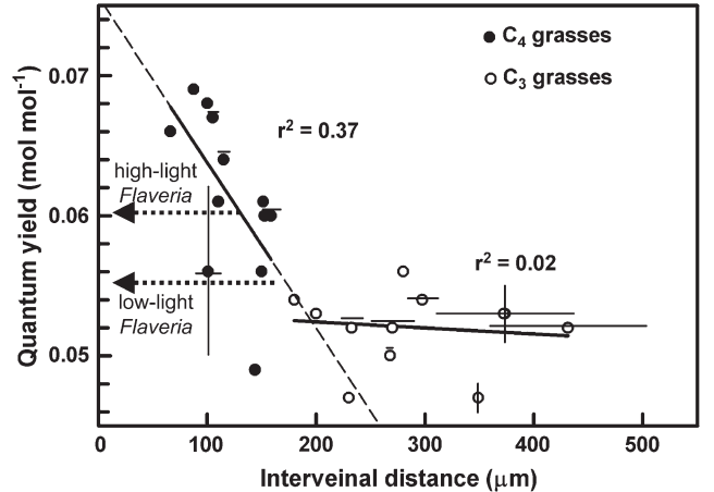
Fig. 3. The relationship between quantum yield and interveinal distance in a variety of C 4 grass species (from Ogle, 2003; with kind permission of Springer Science and Business Media). The horizontal arrows indicate the quantum yield that would correspond to the measured IVD values in Fig. 5C from Flaveria australasica sampled in high light or low light.
