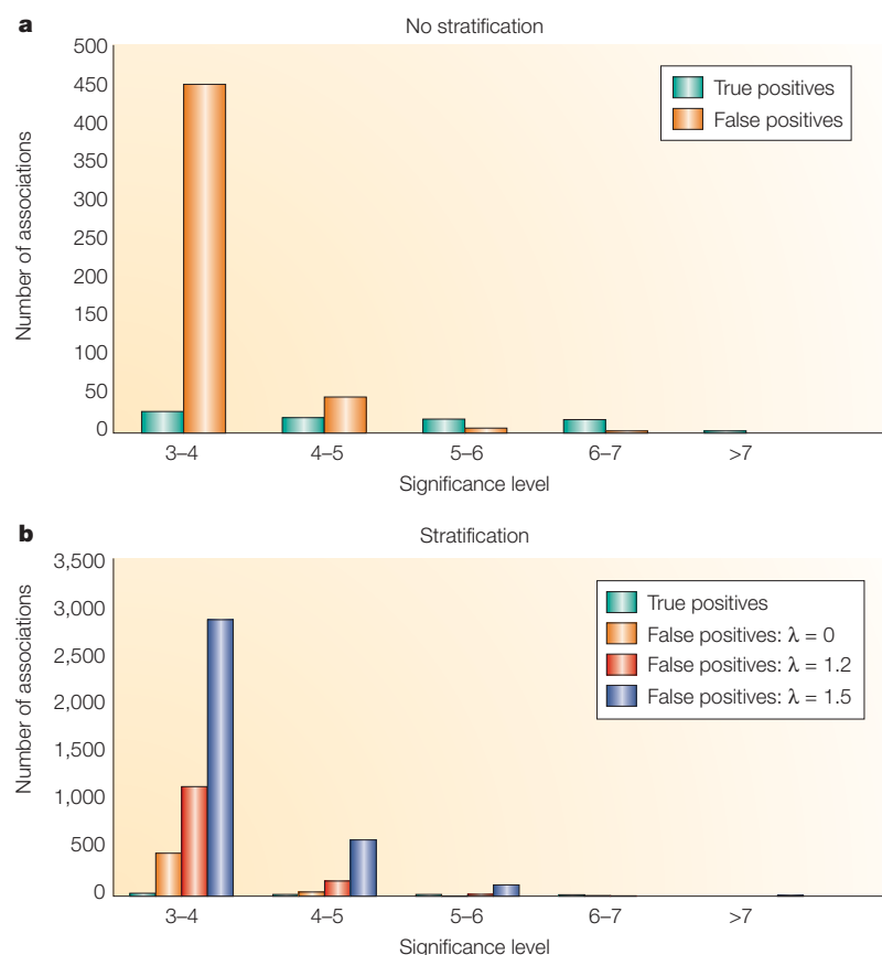
Figure 3 | Effects of population stratification in whole-genome association studies. a A simulation of the effect of population stratification on the ratio of true-positive and false-positive results in a genome-wide association study. a | The expected number of false-positive and true-positive associations detected in a simulated genome-wide association study at different significance levels (shown as the negative log of p -values). Results are shown for a simulated study of 1,000 cases and 1,000 controls, for which 500,000 independent tests are carried out but only 100 represent true associations, with allele frequencies of 15% and odds ratios ranging from 1.2 to 1.5. b | The same scenario is simulated under two different levels of mild stratification, \lambda = 1.2 and \lambda = 1.5 (that is, modelling degrees of stratification such that the typical chi-square statistic for association is inflated by either 1.2 or 1.5; see REF. 103). These levels of \lambda for studies of 1,000 cases and controls are plausible on the basis of recent empirical studies 106 . We modelled the effect of stratification on false-positives by simulating association results under the scenario of no stratification and no true effects and then multiplying the simulated chi-square statistics by a factor of \lambda (see REF. 104).
