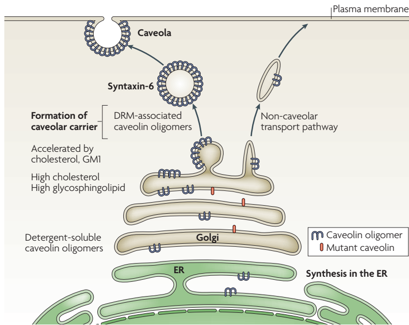
Figure 2 | Caveolin biosynthesis and trafficking to the plasma membrane. Caveolin is synthesized in the endoplasmic reticulum (ER) and is then transported to the Golgi complex as detergent-soluble oligomers. When caveolin exits the Golgi complex, the oligomers associate with glycosphingolipid- and cholesterol-enriched lipid-raft domains, as judged by detergent-resistant membrane (DRM) association. Caveolar carriers that contain quanta of caveolin are produced and fuse directly with the plasma membrane in a process that requires the SNARE protein syntaxin-6. In addition, we propose that caveolin can be transported to the plasma membrane by other carriers. Many caveolin mutants that have been associated with disease conditions accumulate in the Golgi complex and are not transported to the plasma membrane efficiently 135 (as indicated by mutant caveolin (red) in the figure). Expression of these mutants seems to cause a more complete block in Golgi exit, and be more harmful, than total loss of caveolin 37,139,140 . One explanation for this is that proteins that exit the Golgi through the caveolar pathway are facilitated by caveolin, but can also follow other pathways, presumably less efficiently, if caveolin is absent. However, caveolin mutants (which cannot form caveolar carriers) perturb the exit pathway and trap their cargo in the Golgi complex so cargo are unable to 'escape' through other routes.
