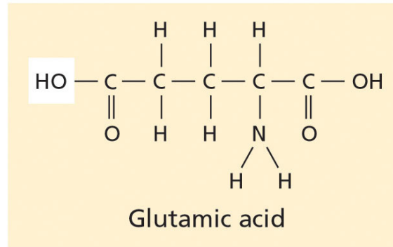
Amino acid
