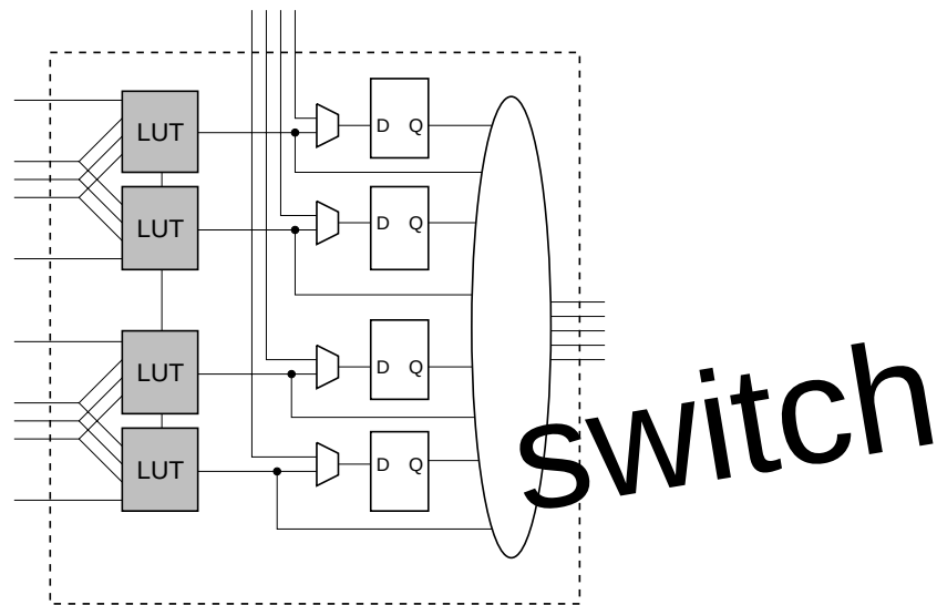
Figure 24 - AT&T Programmable Function Unit (PFU).
