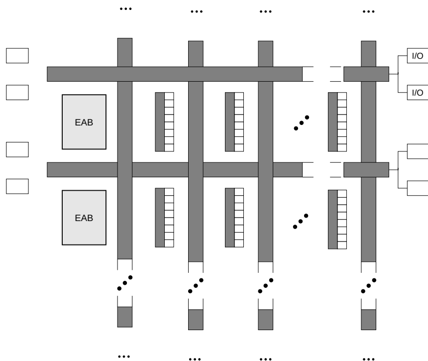
Figure 23 - Architecture of Altera FLEX 10K FPGAs.
