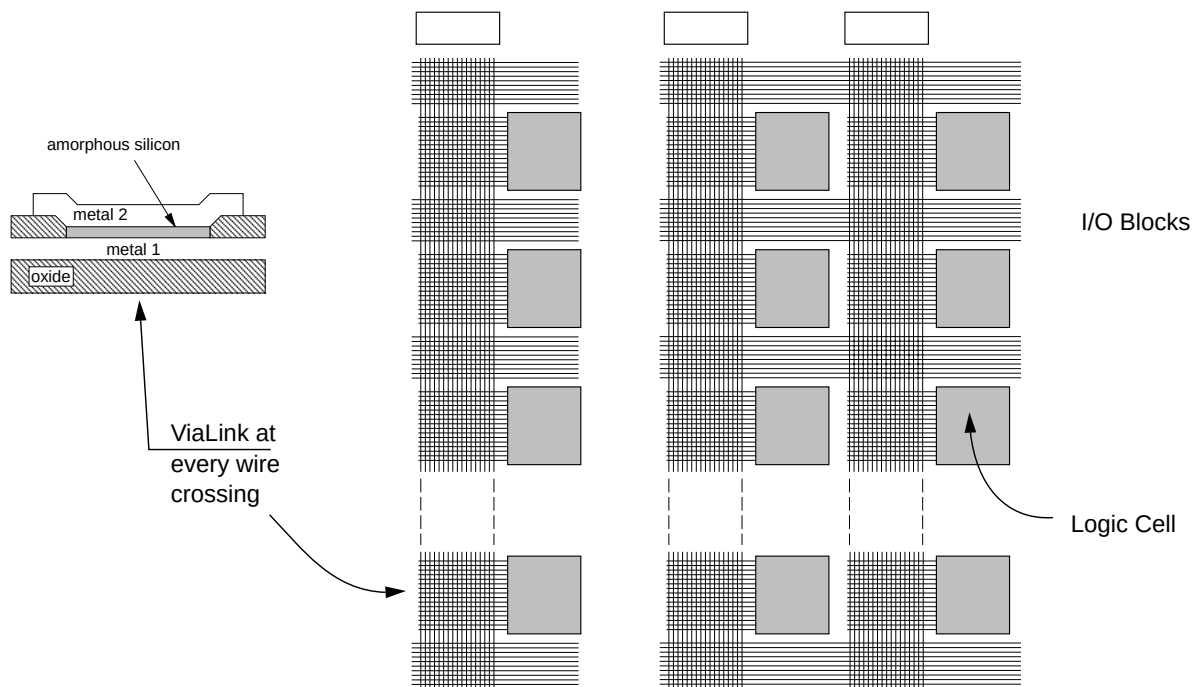
Figure 27 - Structure of Quicklogic pASIC FPGA.
