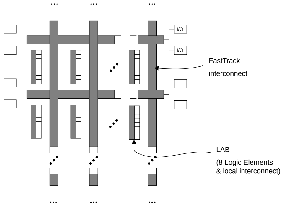
Figure 20 - Architecture of Altera FLEX 8000 FPGAs.
