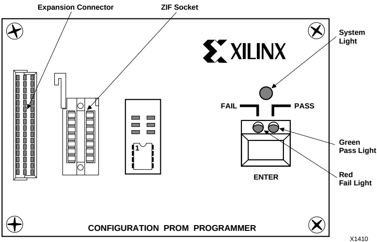
Figure 2-2 HW112 Programmer Top Panel
