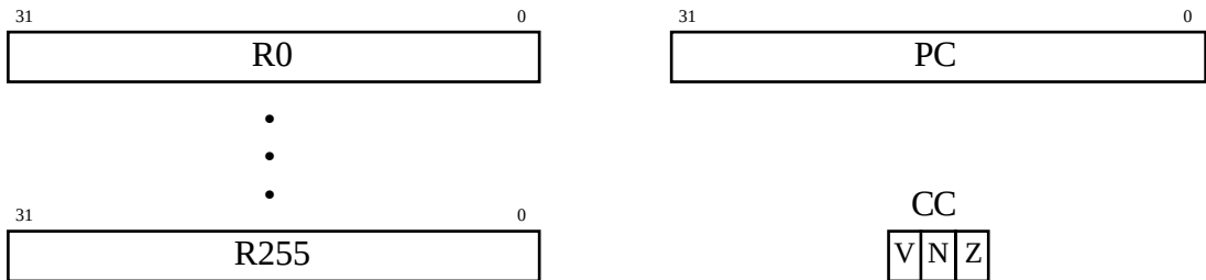
Figure 7-1. DP32 registers.
