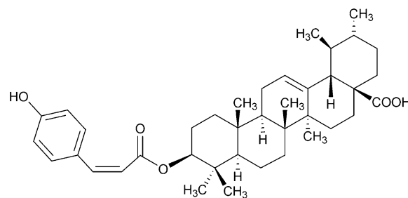
Figure 3 Cis -hydroxycinnamoyl ester of ursolic acid from cranberry fruit.
