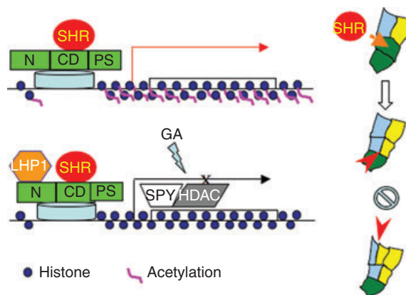
Figure 5. Model depicting the interplay between SCR, GA and the epigenetic machinery in cortex proliferation in the Arabidopsis root. Upon entry into the CEID, SHR together with SCR initially activates cell division genes, but the transcription is rapidly quenched by the interaction between SCR and LHP1, which may be preceded by changes in histone modifications due to other mechanisms. In parallel, GA also suppresses the cell division genes through SPY, which potentially interacts with and modulates the activity of associated HDACs.
