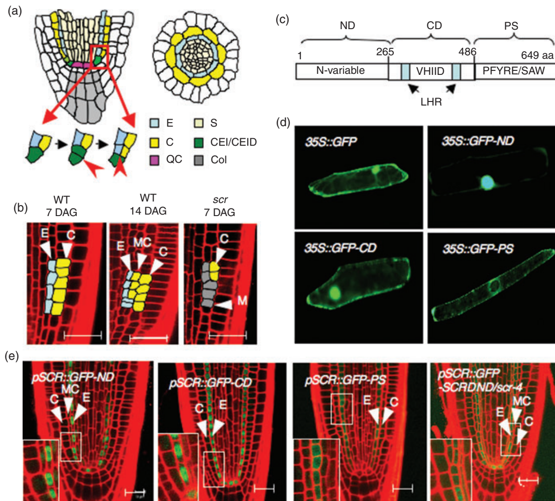
Figure 1. Functional analysis of SCR domains.
