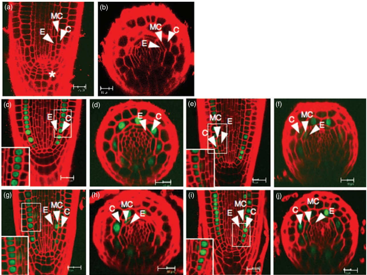
Figure 4. TSA causes premature middle cortex formation.
