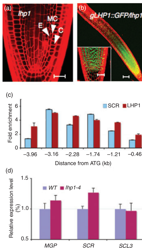
Figure 2. LHP1 acts together with SCR to regulate the timing of middle cortex formation.
